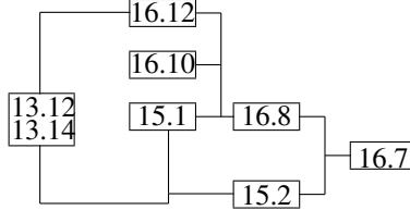
FIGURE 16.1. Scheme of the proof of 16.7
